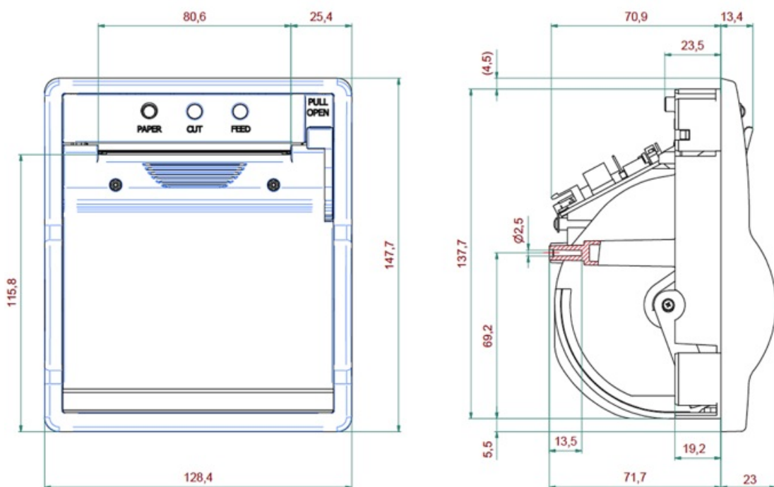
Drawing 2: GeBE-MULDE Naut with paper roll \varnothing 80 mm
